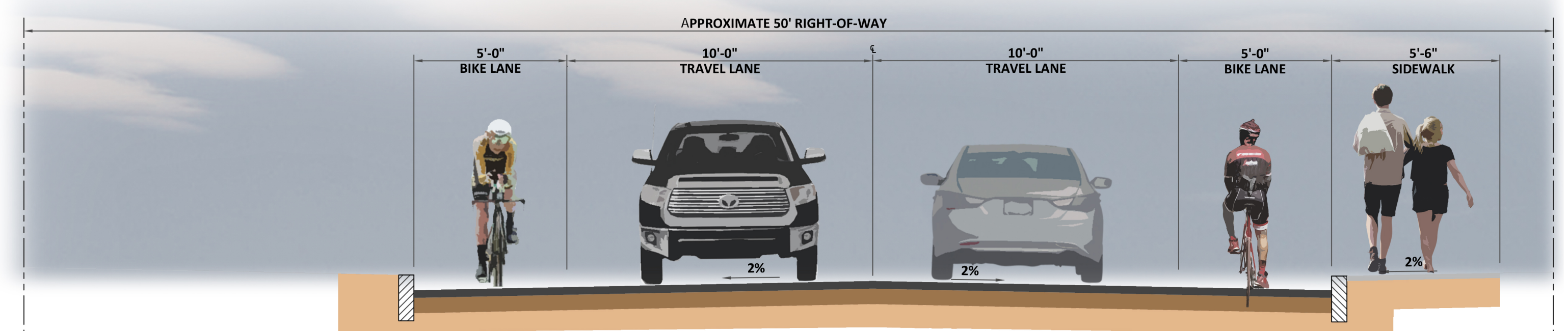
COURT STREET UNION STREET TO HUBBARD ROAD
