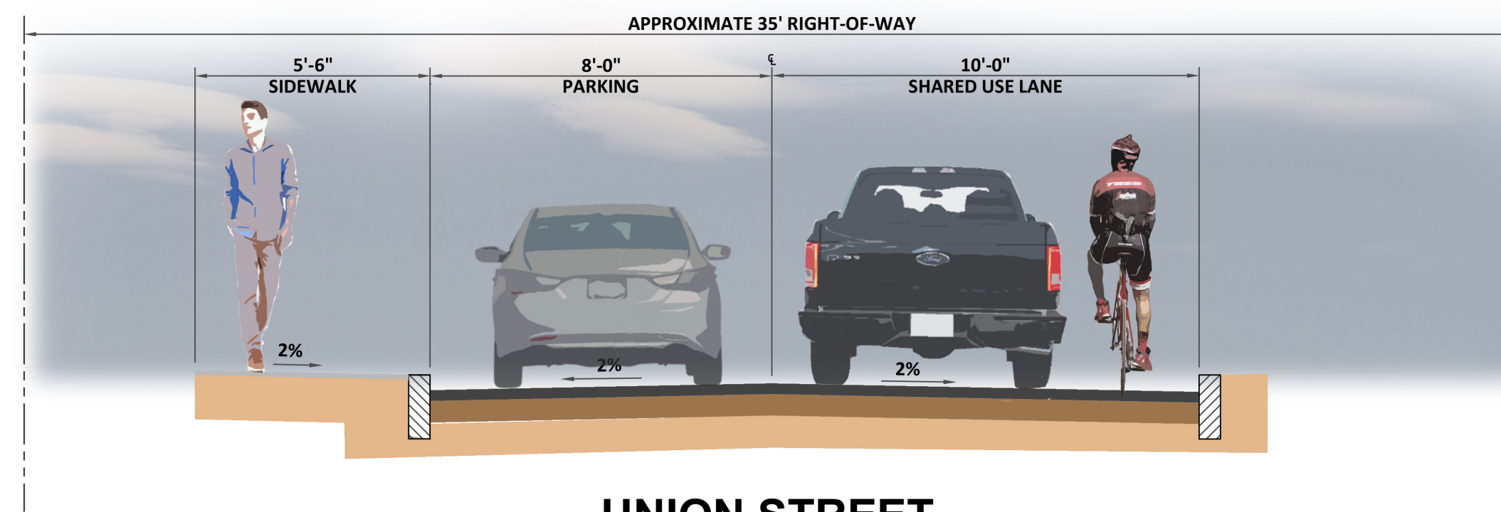
UNION STREET CENTRAL AVENUE TO COURT STREET TYPICAL SECTION
