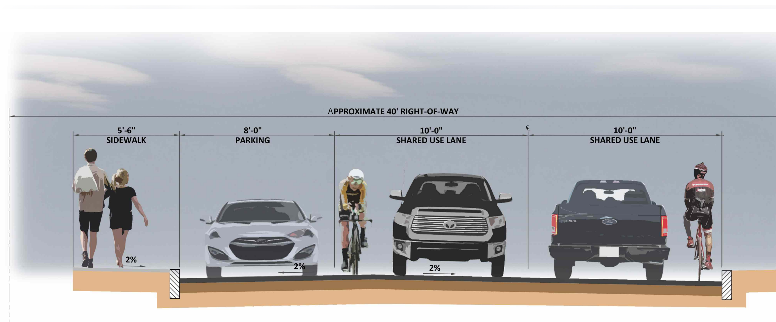
COURT STREET BOYLE STREET TO UNION STREET
